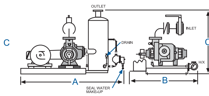
Recirculated Seal, V-Belt Drive
