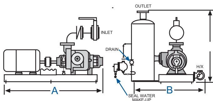
Recirculated Seal, Direct Drive
